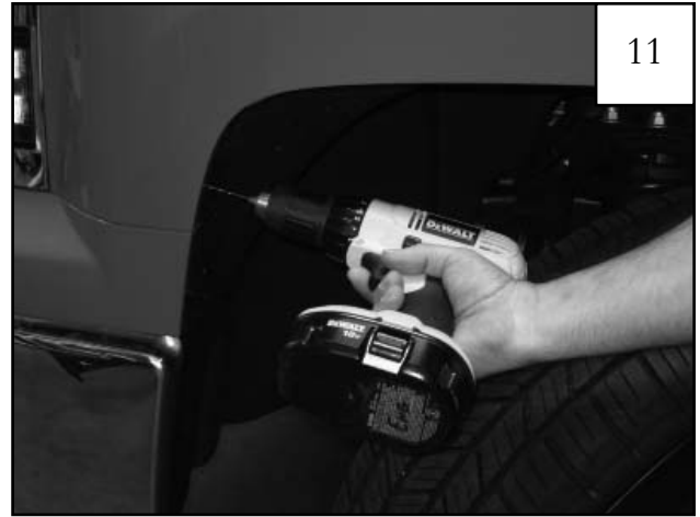
Using a 3/32" drill bit, drill pilot holes at the marks made in Step 9.
