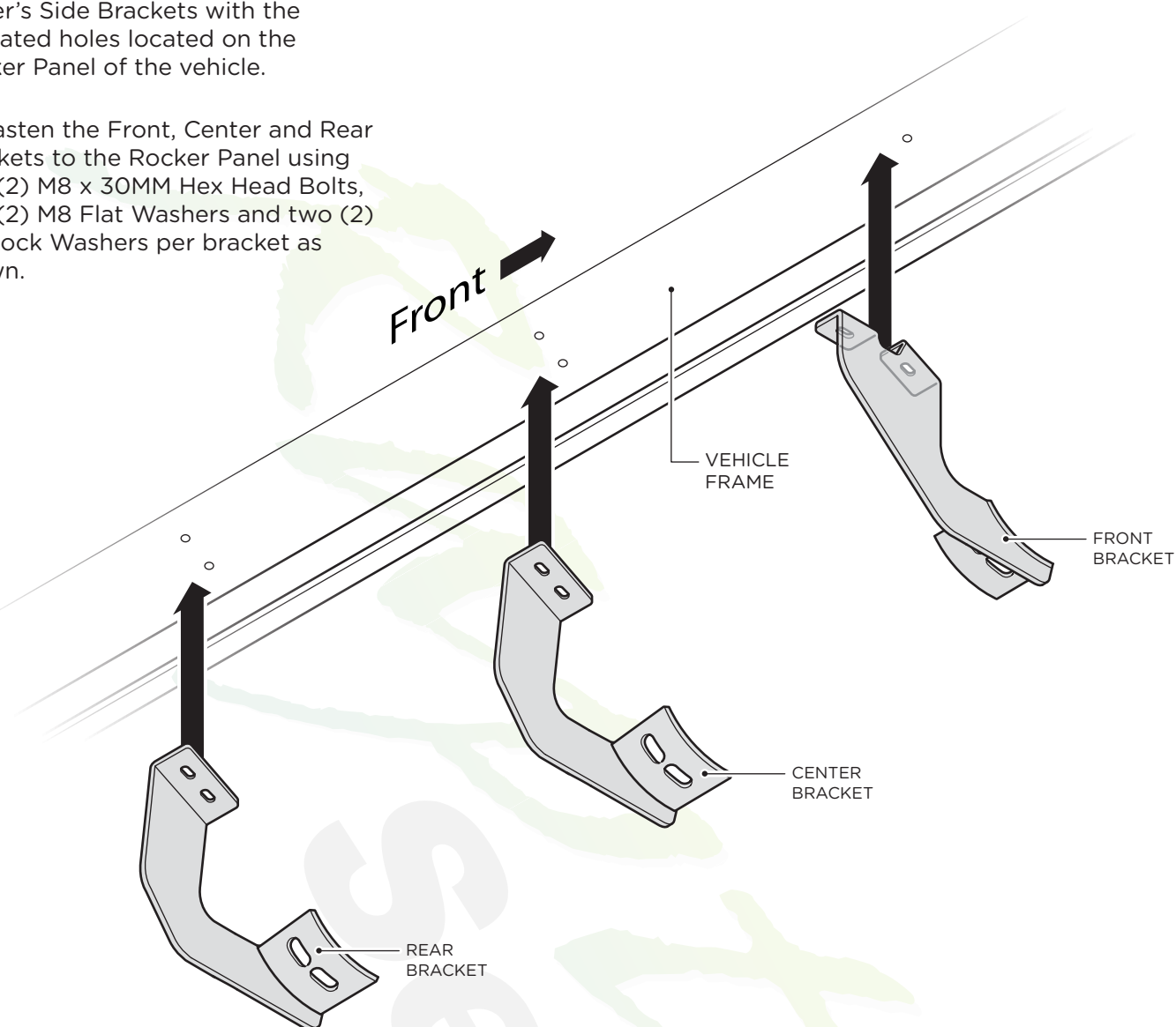
Center & Rear Bracket
