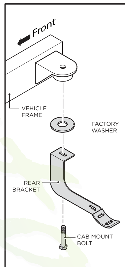
Rear Bracket
