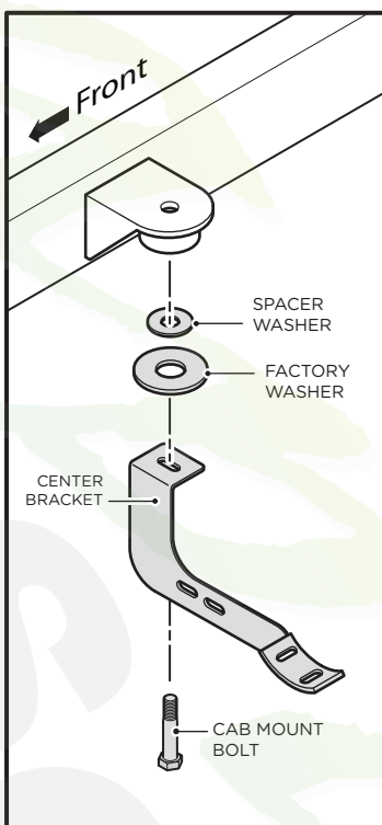
Center Bracket
