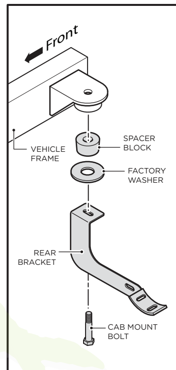
Rear Bracket
