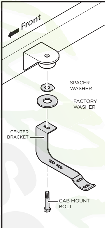
Center Bracket
