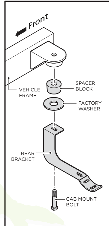
Rear Bracket
