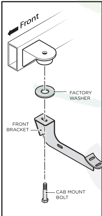
Front Bracket
