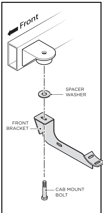
Front Bracket
