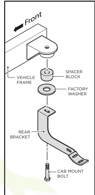
Rear Bracket
